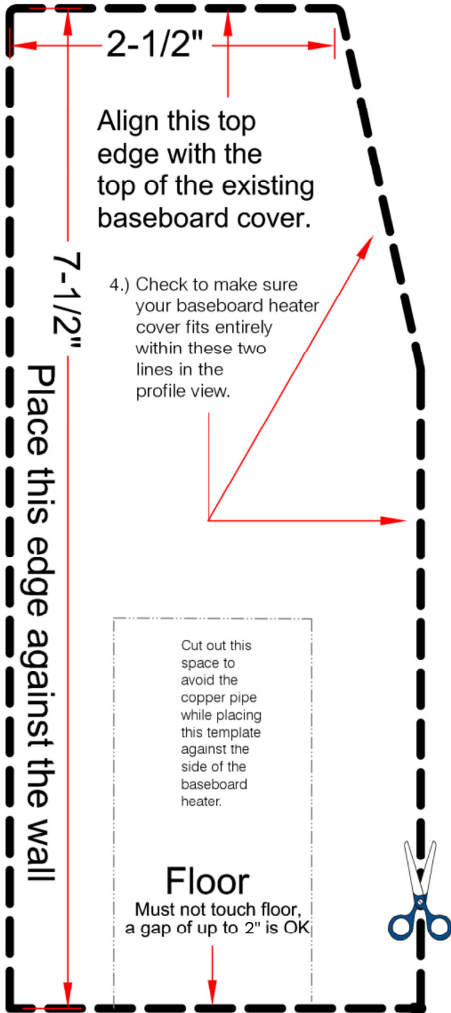
Profile View of an Endcap
